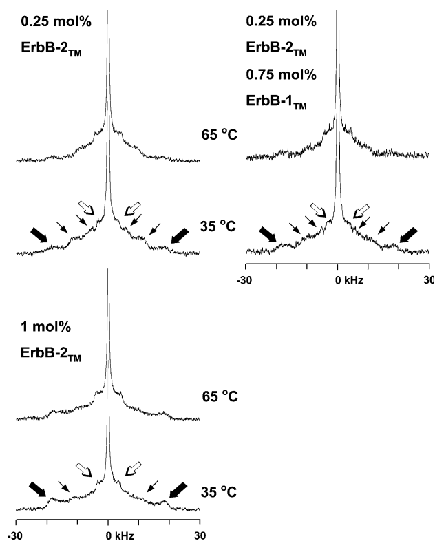
Fig. 2. 2 H NMR spectra corresponding to ErbB-2 TM at low receptor concentration. Arrayed spectra are displayed for ErbB-2 TM at 0.25 and 1 mol% in POPC bilayers (left). Also shown are spectra for ErbB-2 TM in POPC bilayers containing 0.75 mol% unlabelled ErbB-1 TM (right). Thick solid arrows indicate the 38.5 kHz splitting arising from peptide rotating \ll 10^5 s -1 (presumed oligomers); thin arrows indicate spectral features attributed to dimers and/or small oligomers capable of rotation faster than 10^5 s -1 ; hollow arrows indicate narrowed Pake doublets associated with peptides whose rotational diffusion \gg 10^5 s -1 (presumed monomers). Typically 800 000–1 000 000 transients were accumulated for each spectrum.
